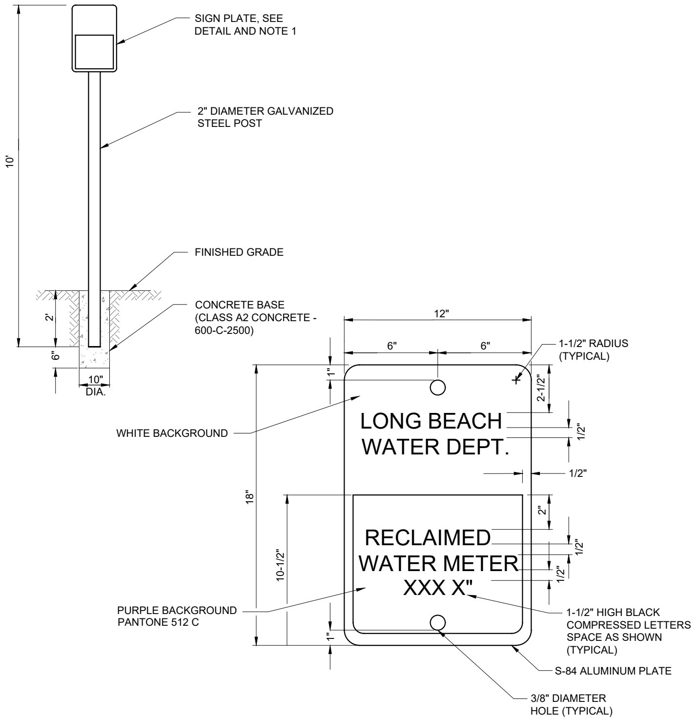
SIGN PLATE DETAIL
