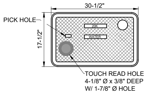
METER COVER
