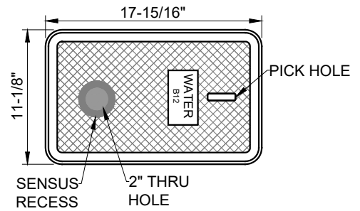
METER COVER
