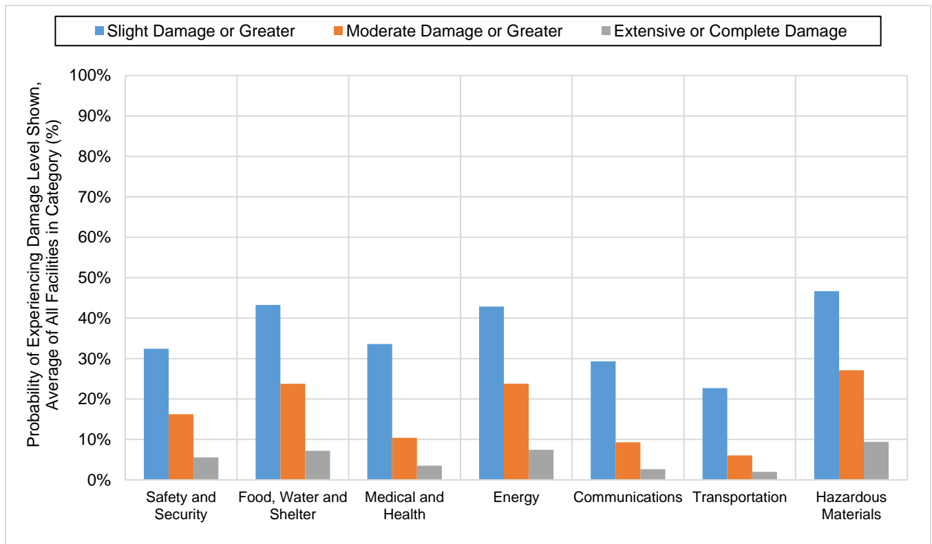
Figure 8-13. Critical Facility Damage Potential, 100-Year Probabilistic Earthquake
