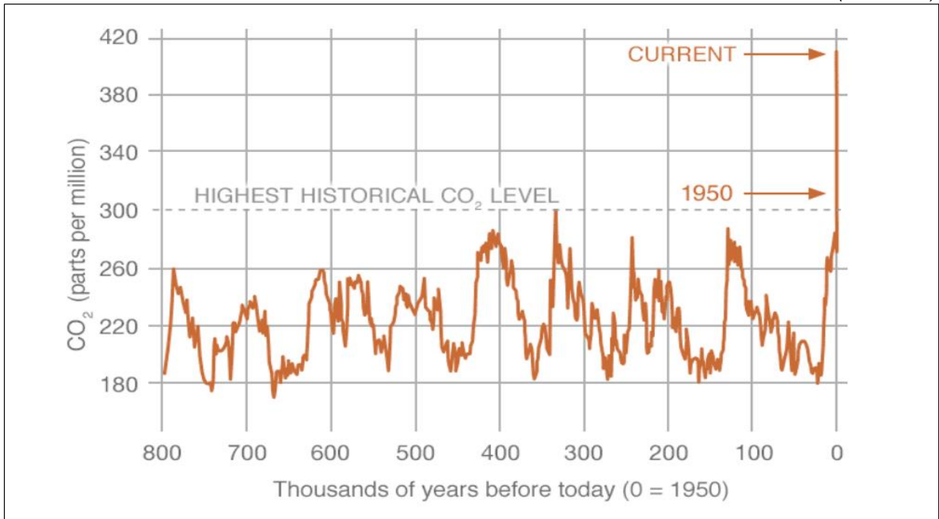
Figure 13-1. Global Carbon Dioxide Concentrations Over Time
