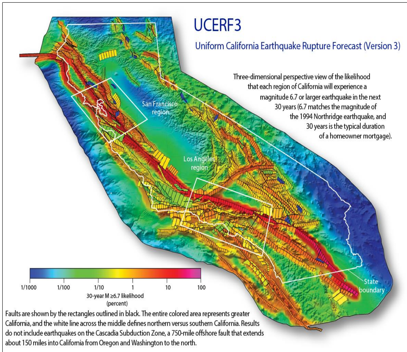
Figure 8-4. UCERF3 Forecast for Magnitude 6.7 or Larger Earthquake in the Next 30 Years
