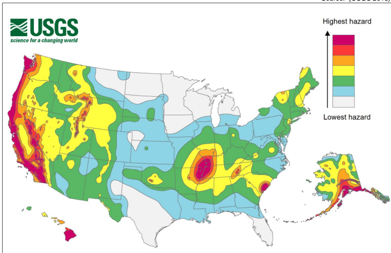
Figure 8-1. 2018 USGS National Seismic Hazard Map
