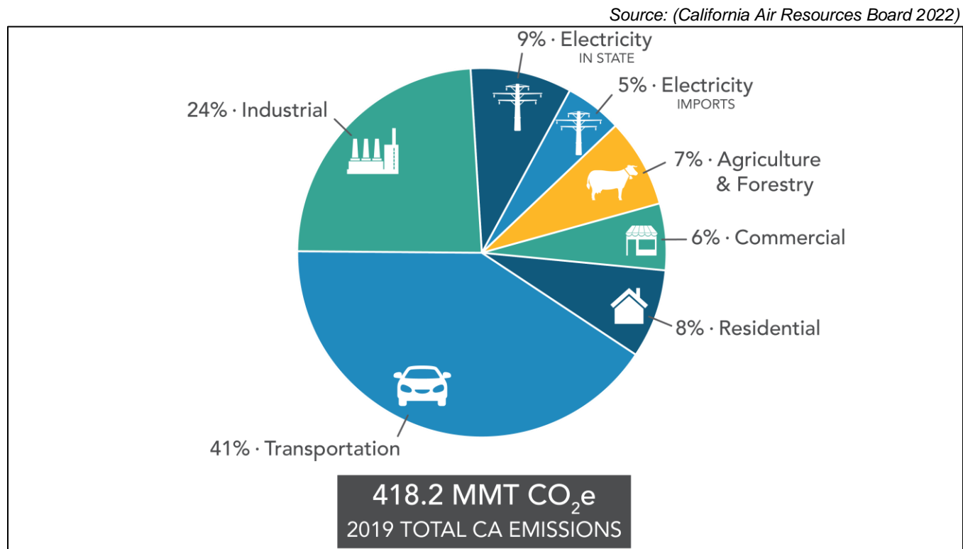
Figure 13-2. California’s 2019 Greenhouse Gas Emission Inventory by Sector
