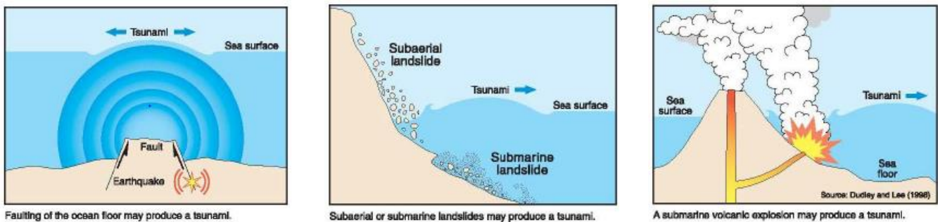
Figure 12-1. Common Sources of Tsunamis
