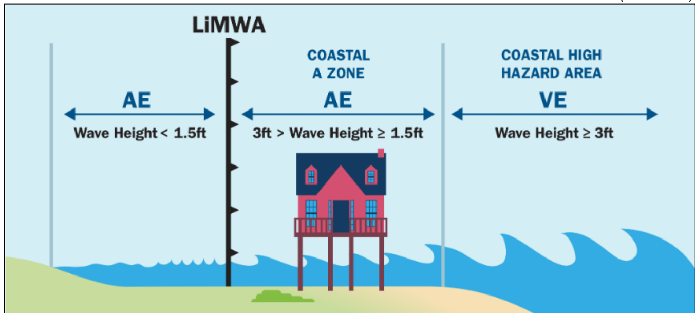
Figure 10-1. Limit of Moderate Wave Action
