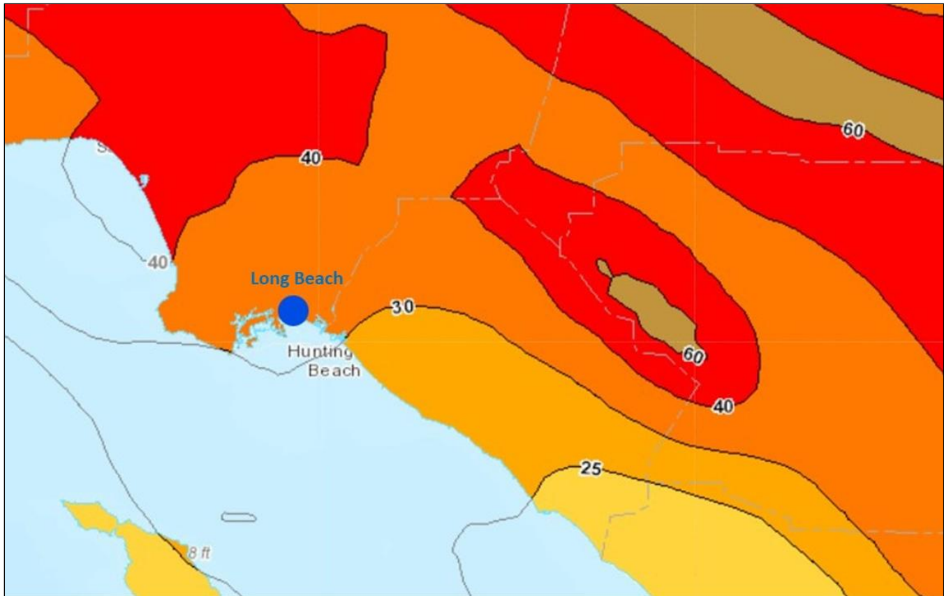
Figure 8-5. PGA with 2-Percent Probability of Exceedance in 50 Years
