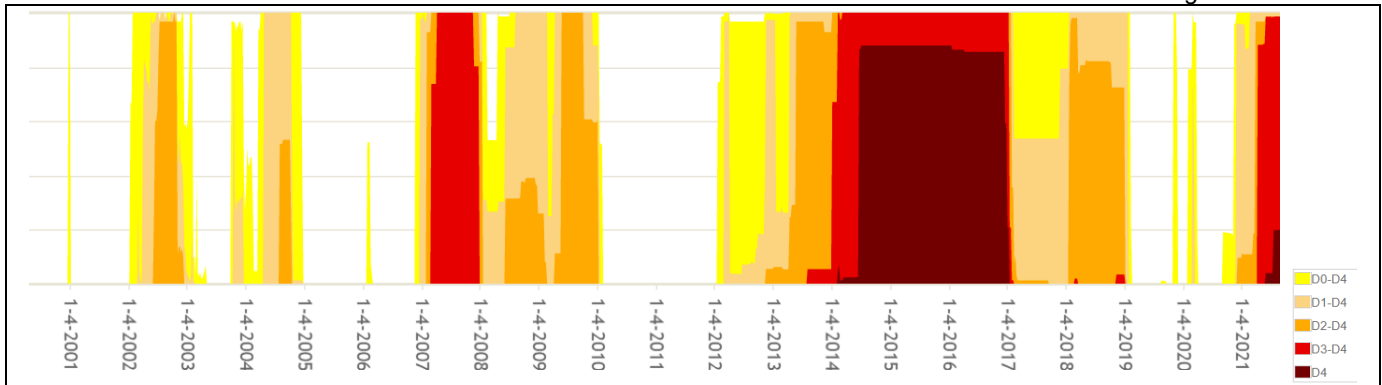
Figure 14-3. Percent of Los Angeles County Affected by USDM Ratings, 2000 –2022
