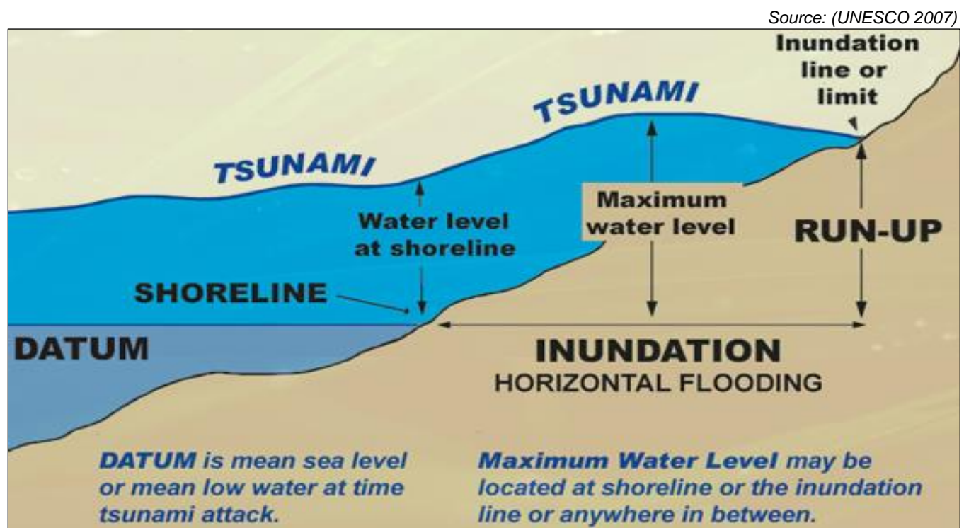
Figure 12-2. Runup Distance and Height in Relation to the Datum and Shoreline
