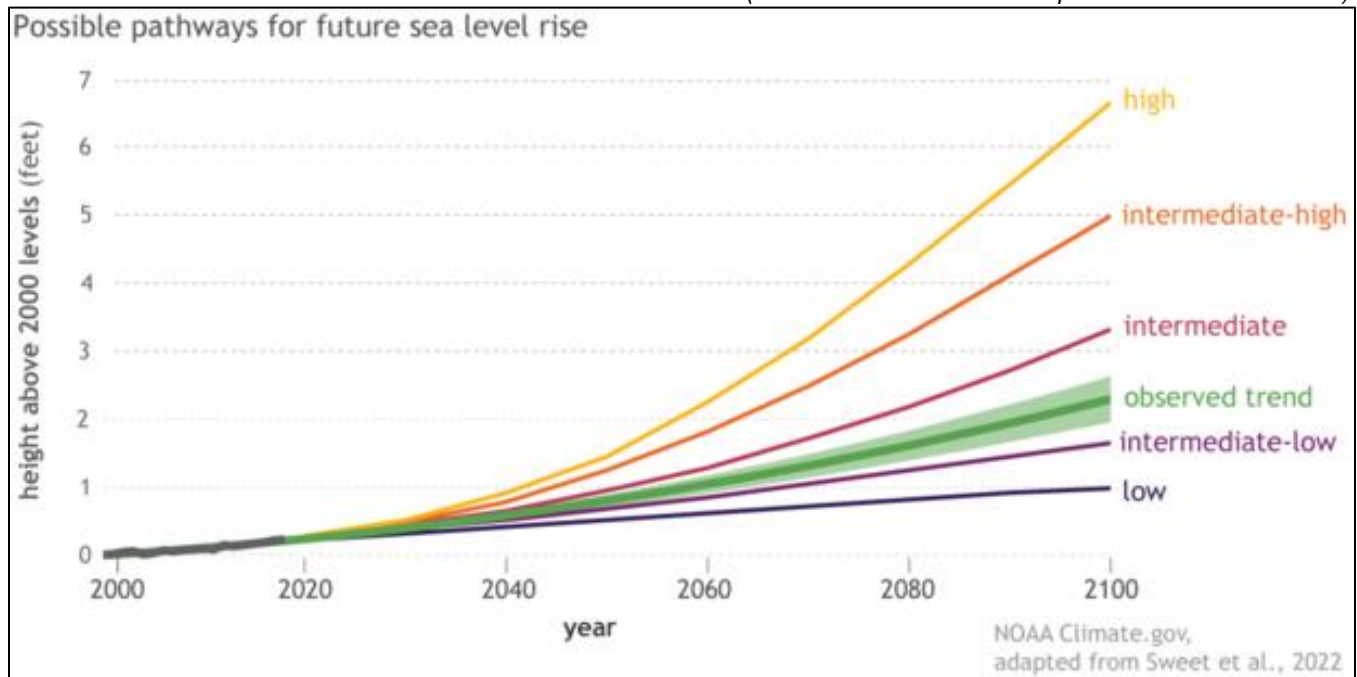
Figure 13-3. Possible Pathways for Future Sea Level Rise
